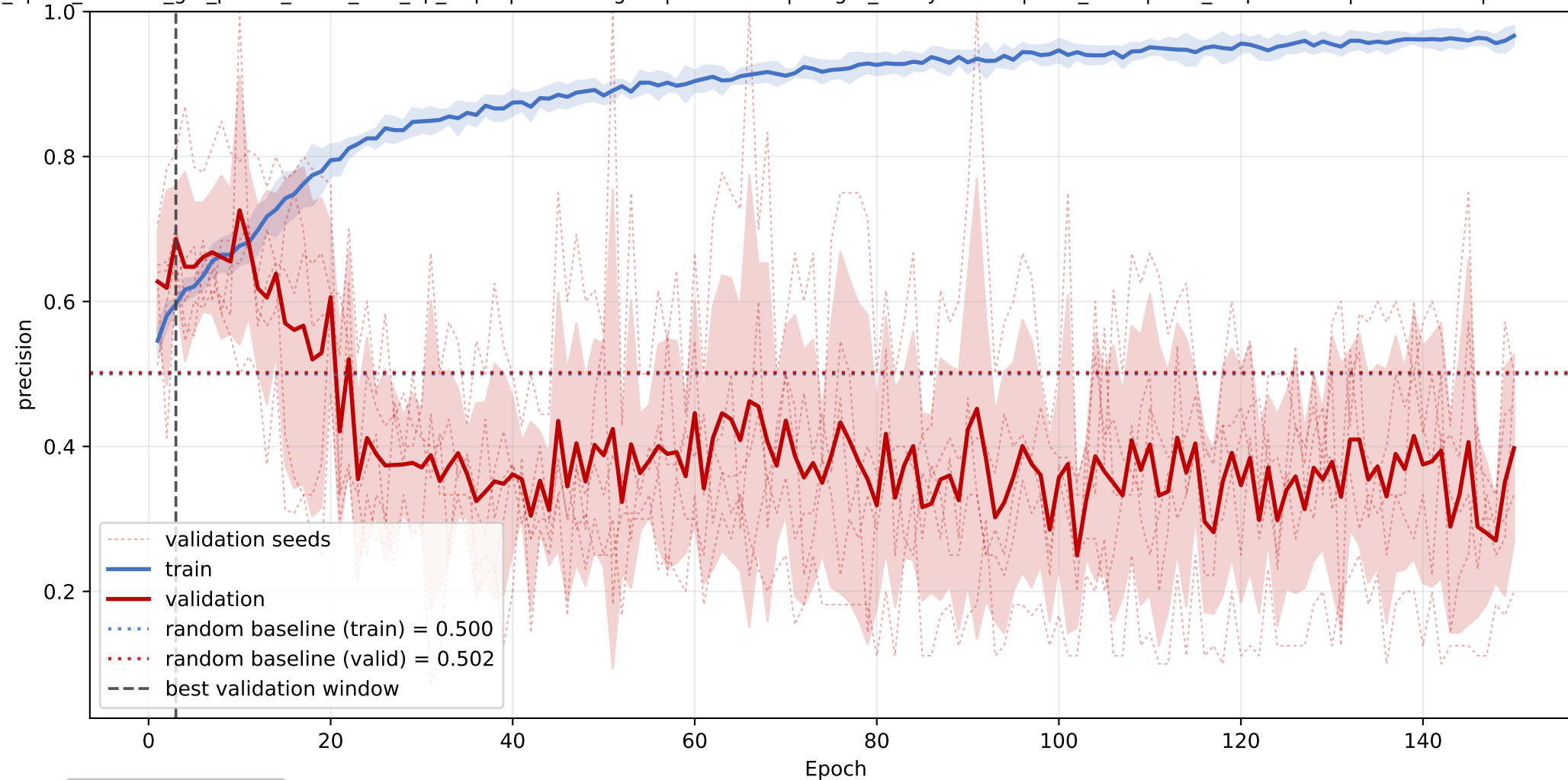
LBP_BPI_CETP: mean precision learning curve across seeds
