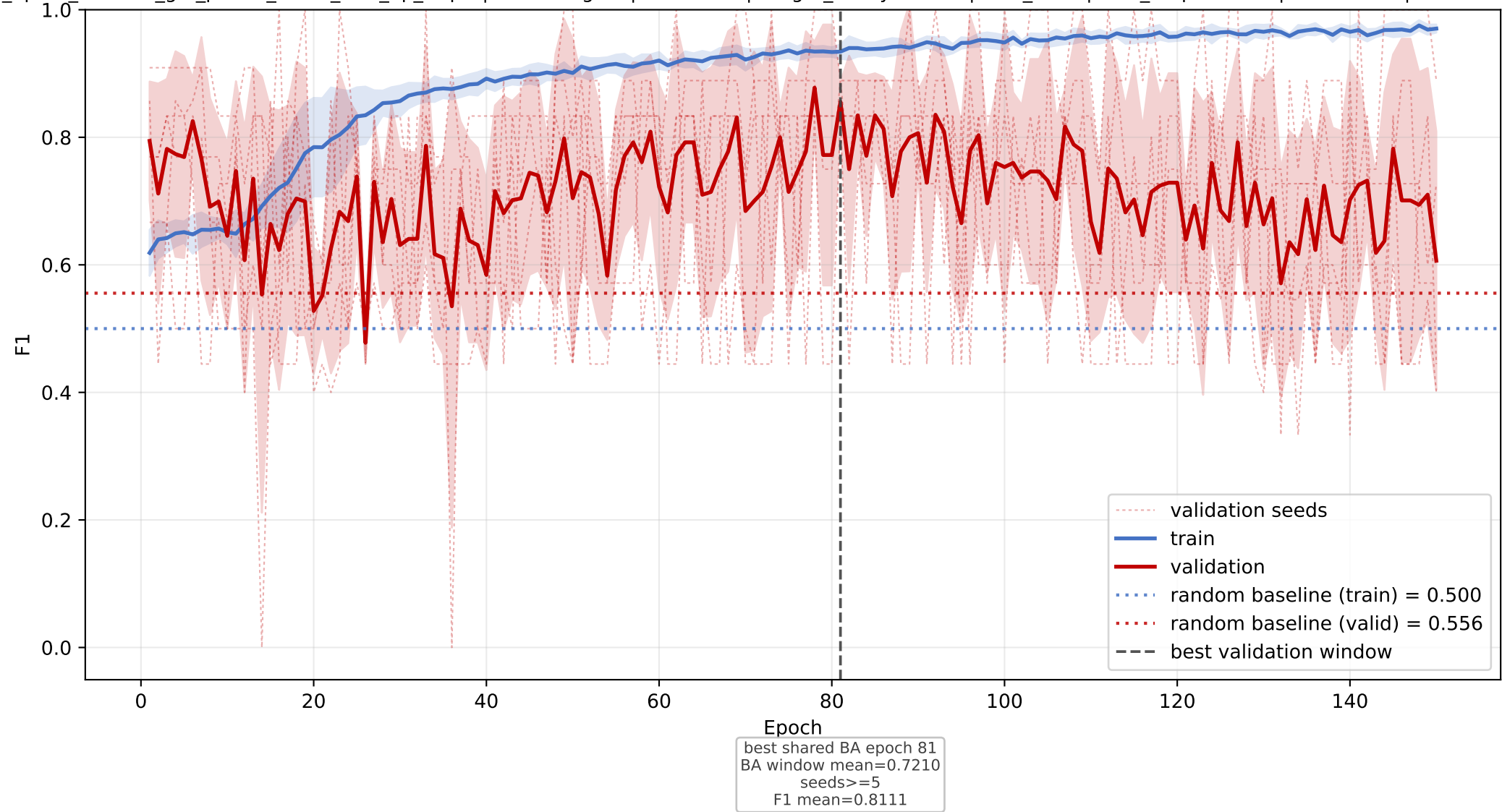
OSBP: mean F1 learning curve across seeds
