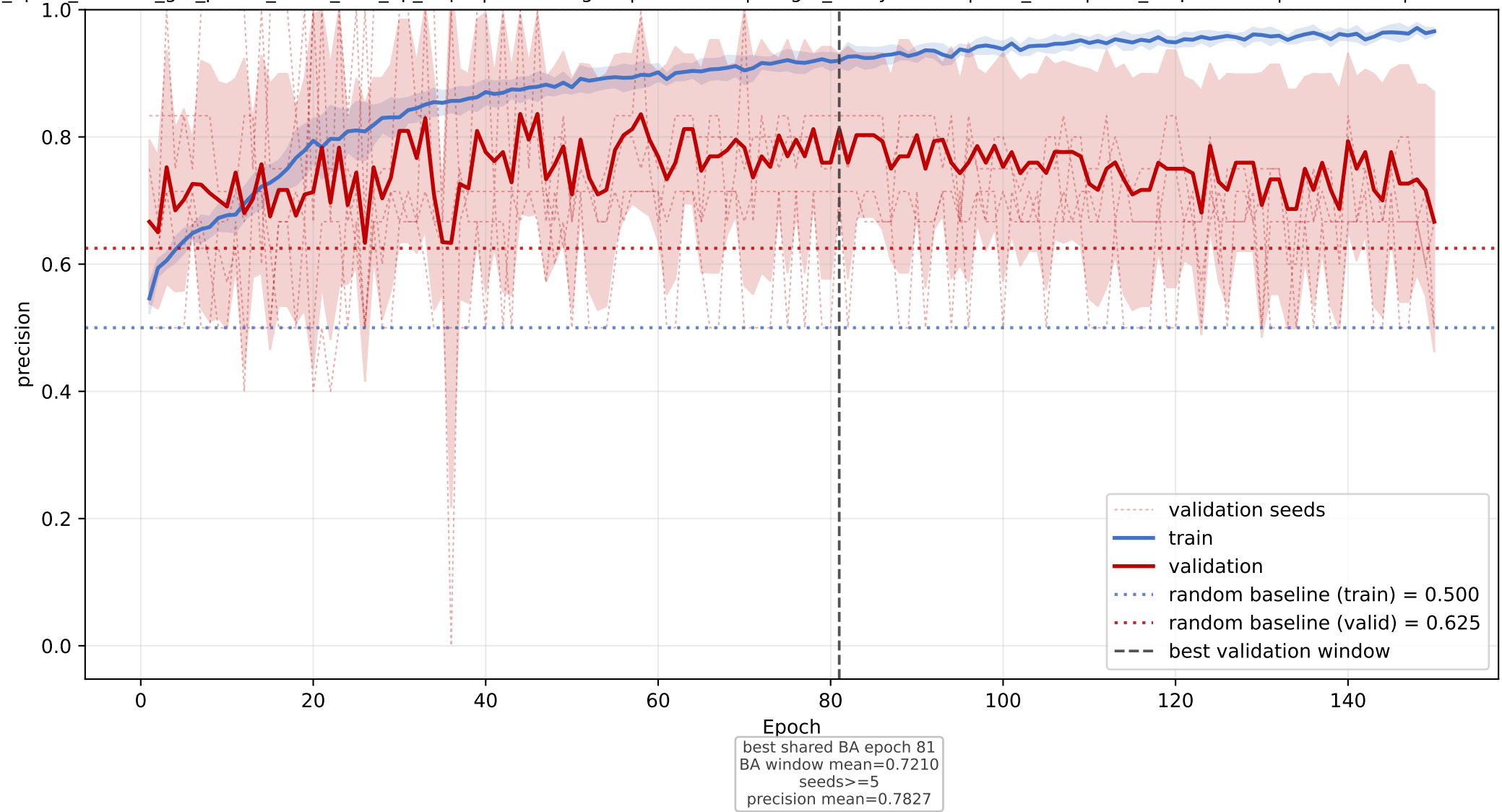
OSBP: mean precision learning curve across seeds
