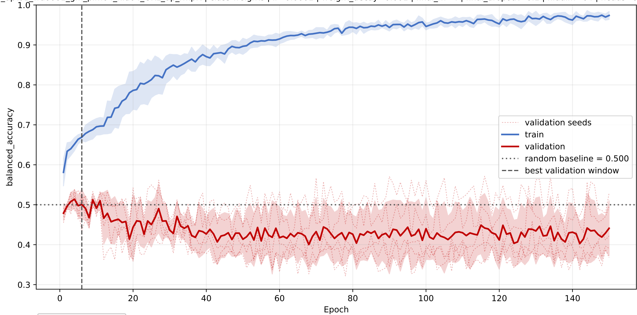
START: mean balanced_accuracy learning curve across seeds
