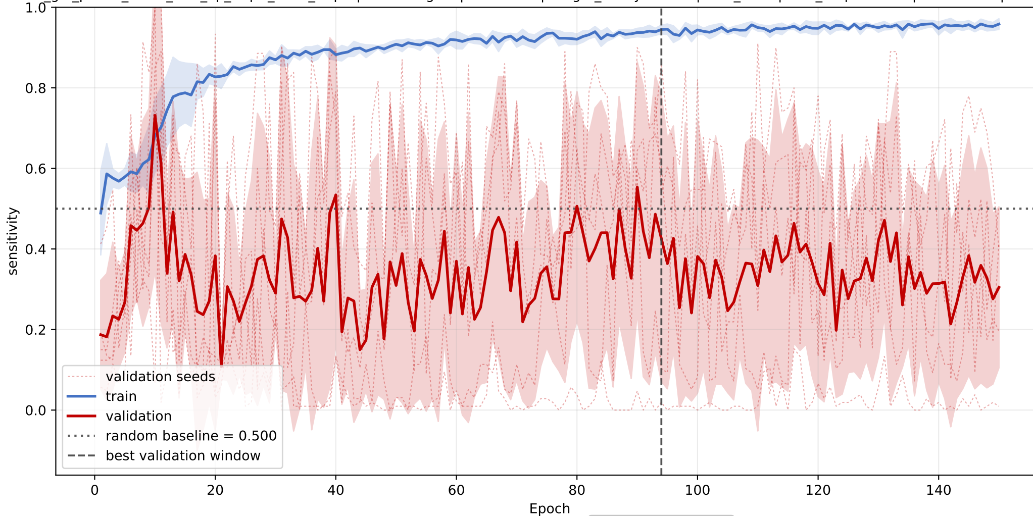
CRAL-TRIO: mean sensitivity learning curve across seeds
