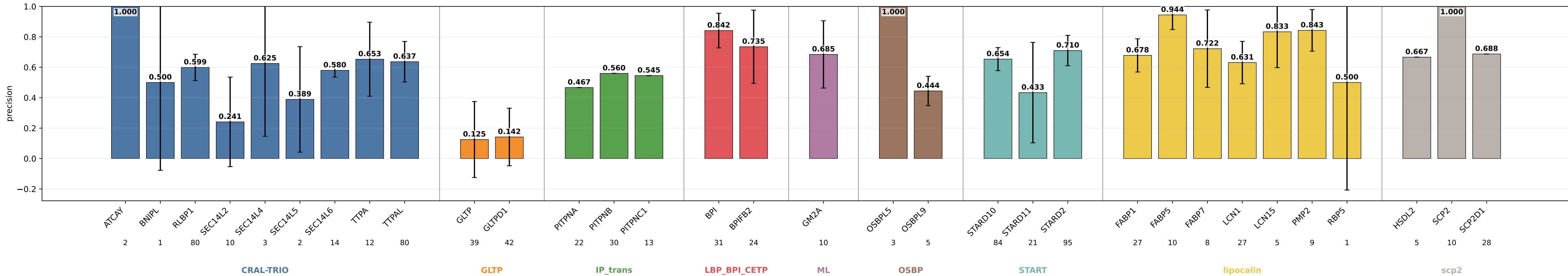
bbp_fa_nps3mlp_dpt01_wd0001_gm_plm64_hid64_GRL_dp_rmpft_dann_rmpft precision by subgroup bbp_fa_nps3mlp_dpt01_wd0001_gm_plm64_hid64_GRL_dp_rmpft_dann_rmpft | class weights | lr=0.0001 | weight_decay=0.001 | final_m=4 | final_dropout=0.1 | hiddim=64 | heads=8 | batch=16 | ep=150 | seeds=0,1,2,3,4
