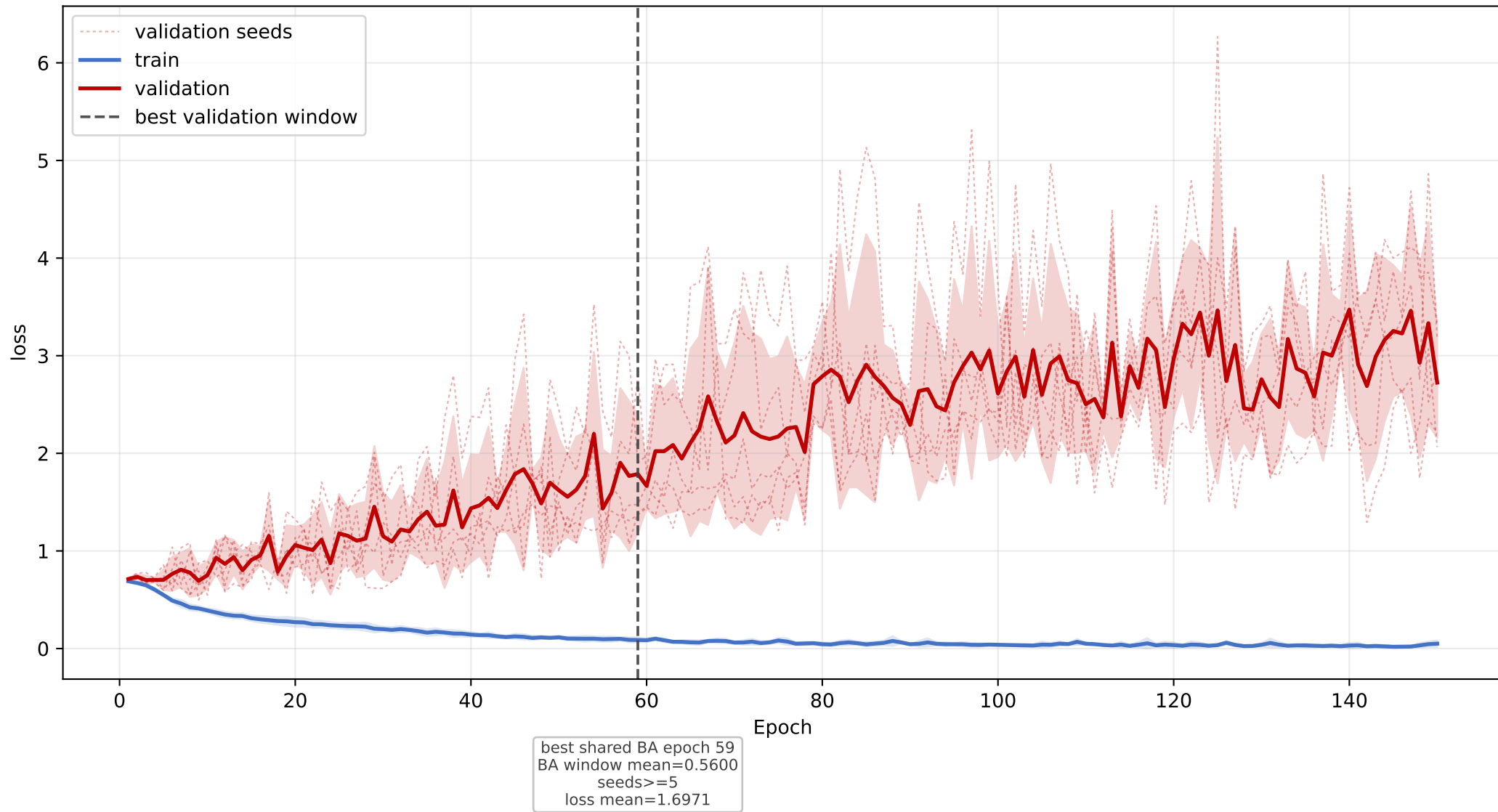
CRAL-TRIO: mean loss learning curve across seeds
