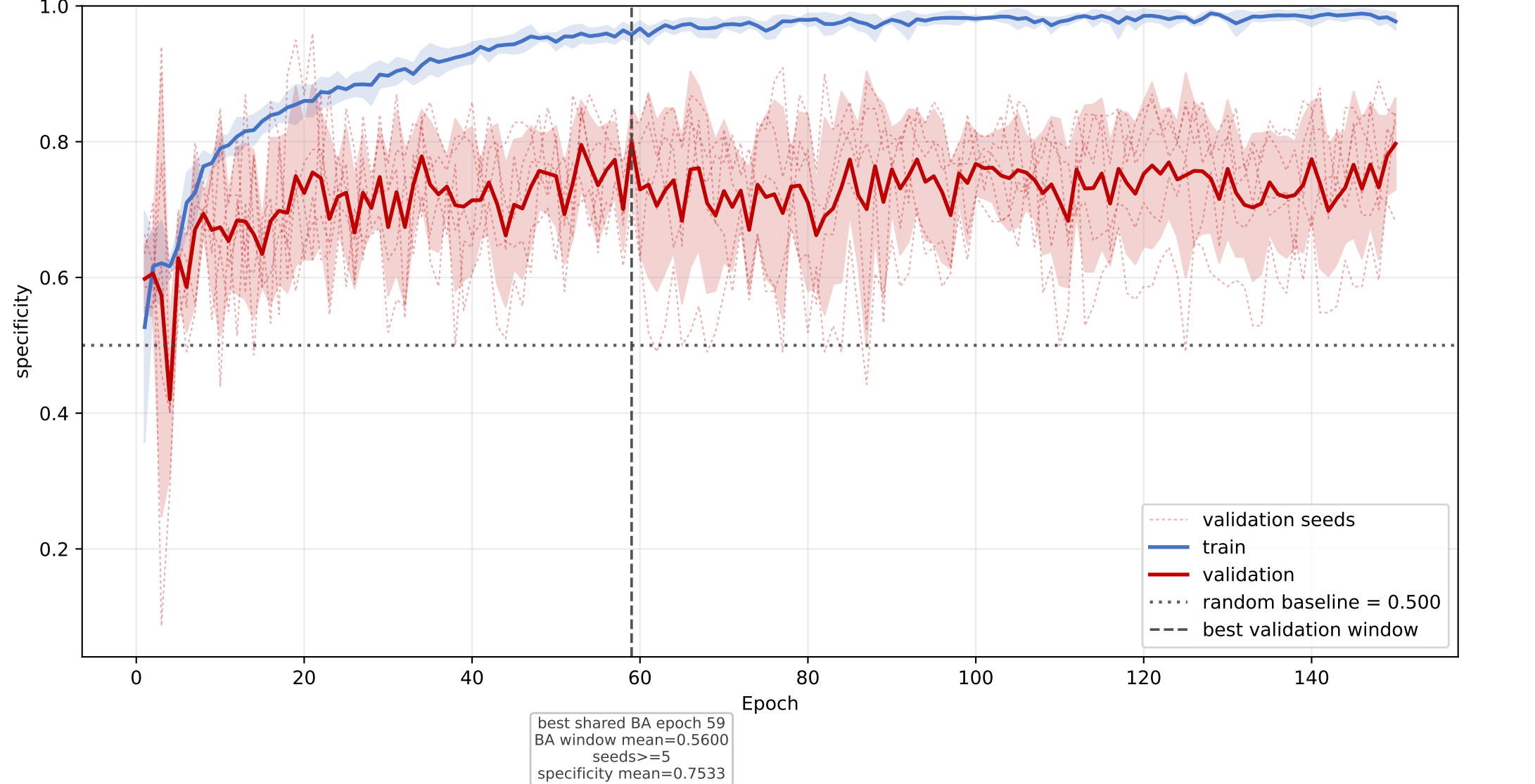
CRAL-TRIO: mean specificity learning curve across seeds
