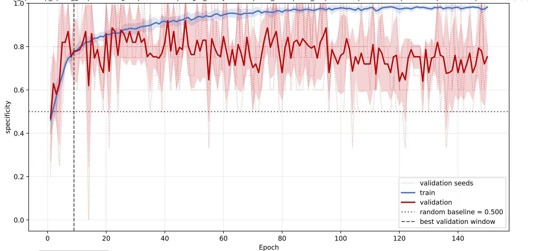
ML: mean specificity learning curve across seeds
