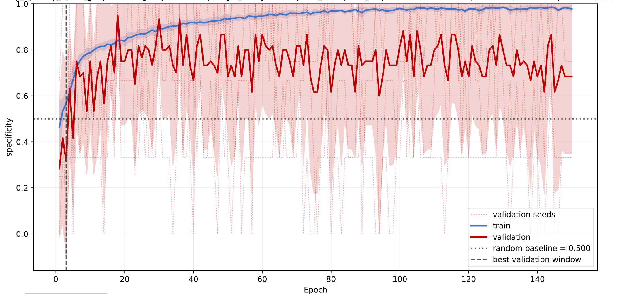
OSBP: mean specificity learning curve across seeds
