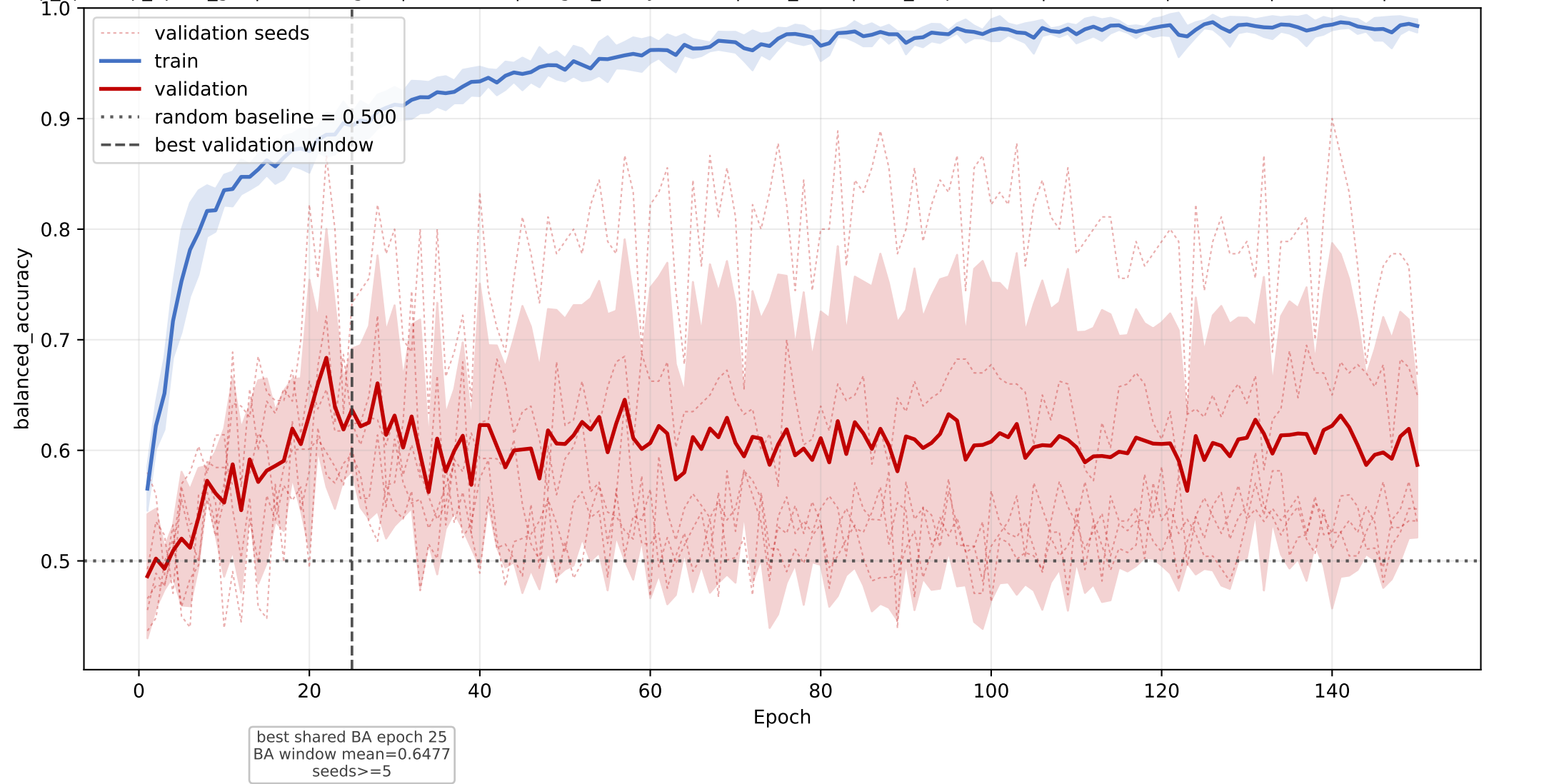
lipocalin: mean balanced_accuracy learning curve across seeds
