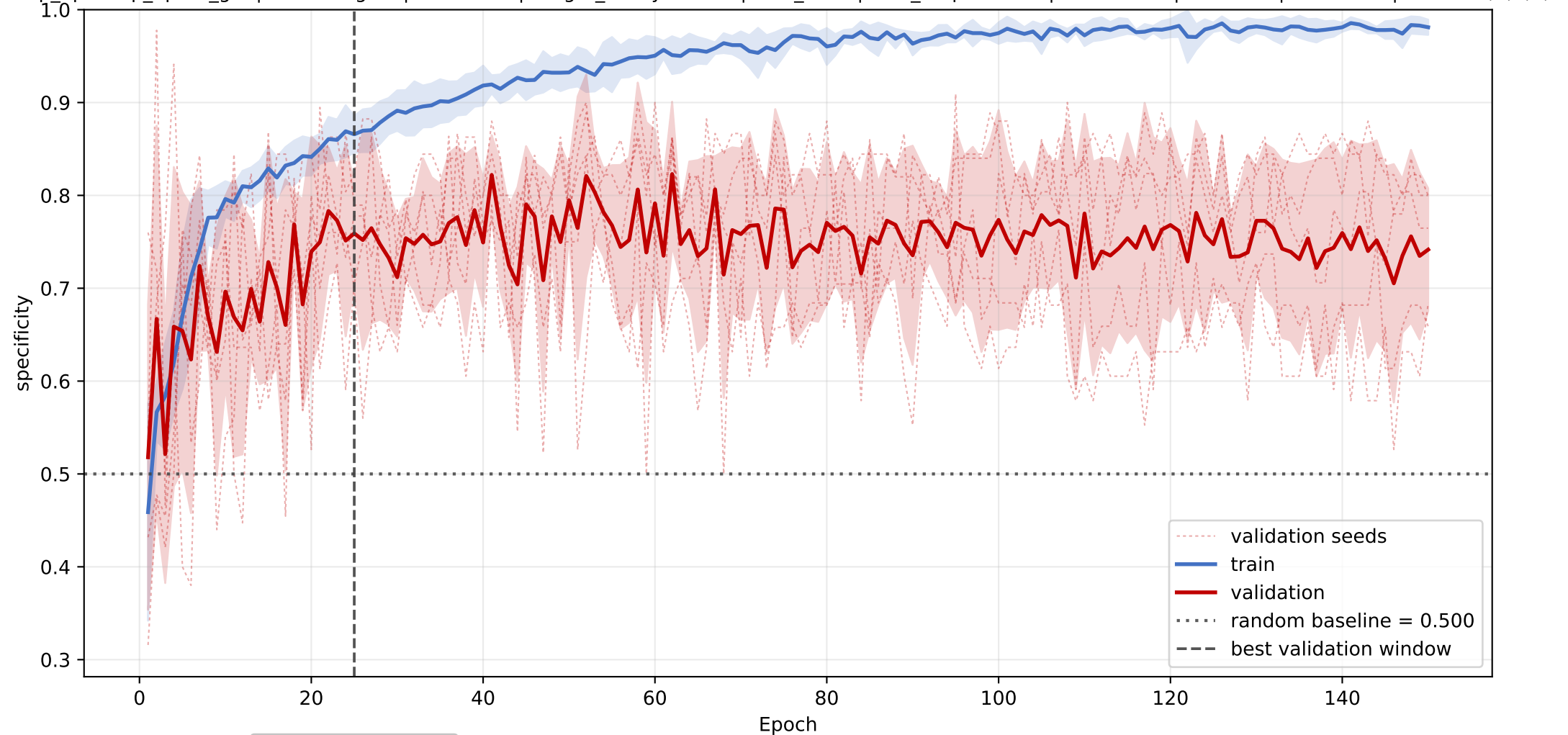
lipocalin: mean specificity learning curve across seeds
