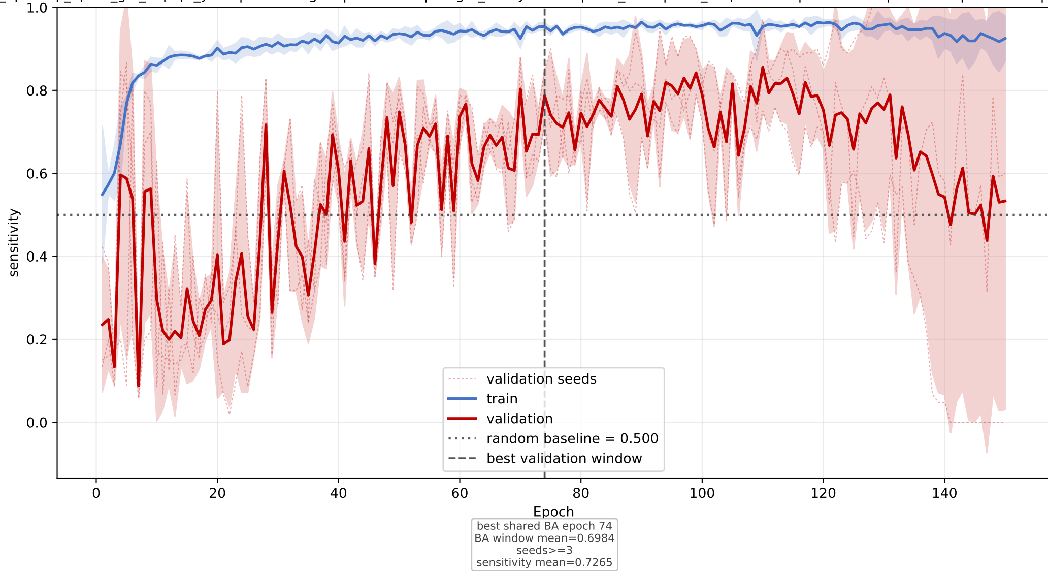
CRAL-TRIO: mean sensitivity learning curve across seeds
