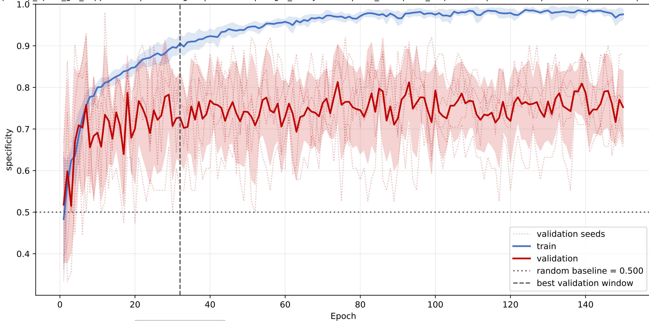
lipocalin: mean specificity learning curve across seeds
