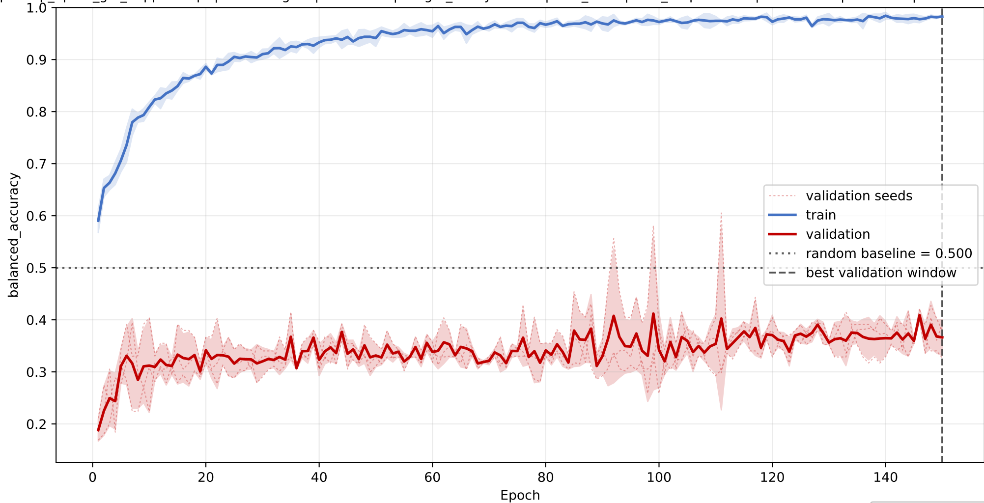
GLTP: mean balanced_accuracy learning curve across seeds
