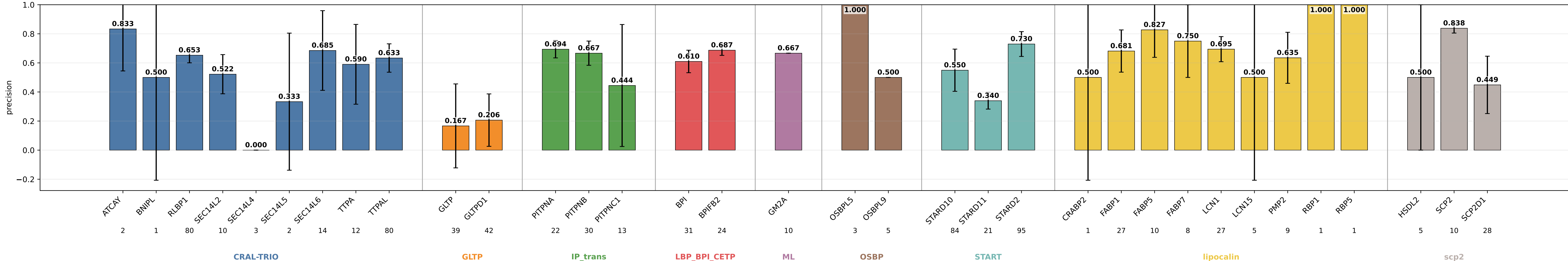
bbp_nps3mlp_dpt01_gm_mlpplm1lopt precision by subgroup bbp_nps3mlp_dpt01_gm_mlpplm1lopt | class weights | lr=0.0001 | weight_decay=1e-05 | final_m=4 | final_dropout=0.1 | hiddim=96 | heads=8 | batch=16 | ep=150 | seeds=0,1,2
