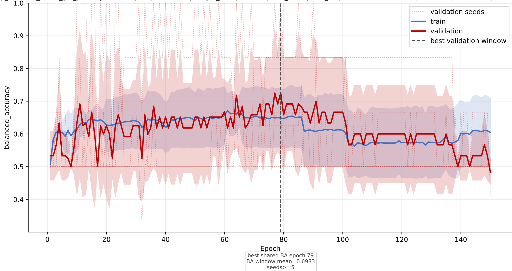
OSBP: mean balanced_accuracy learning curve across seeds
