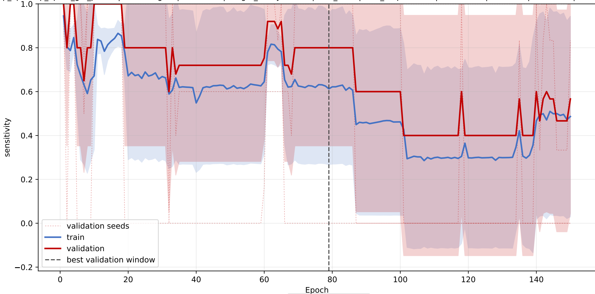
OSBP: mean sensitivity learning curve across seeds
