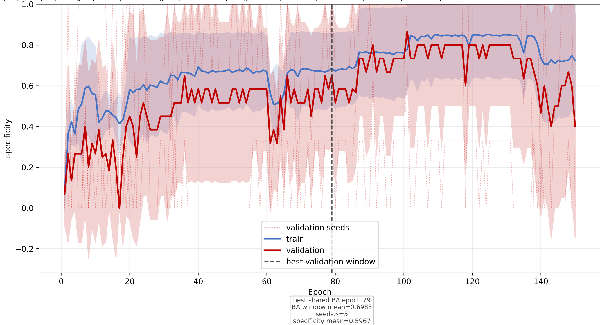
OSBP: mean specificity learning curve across seeds
