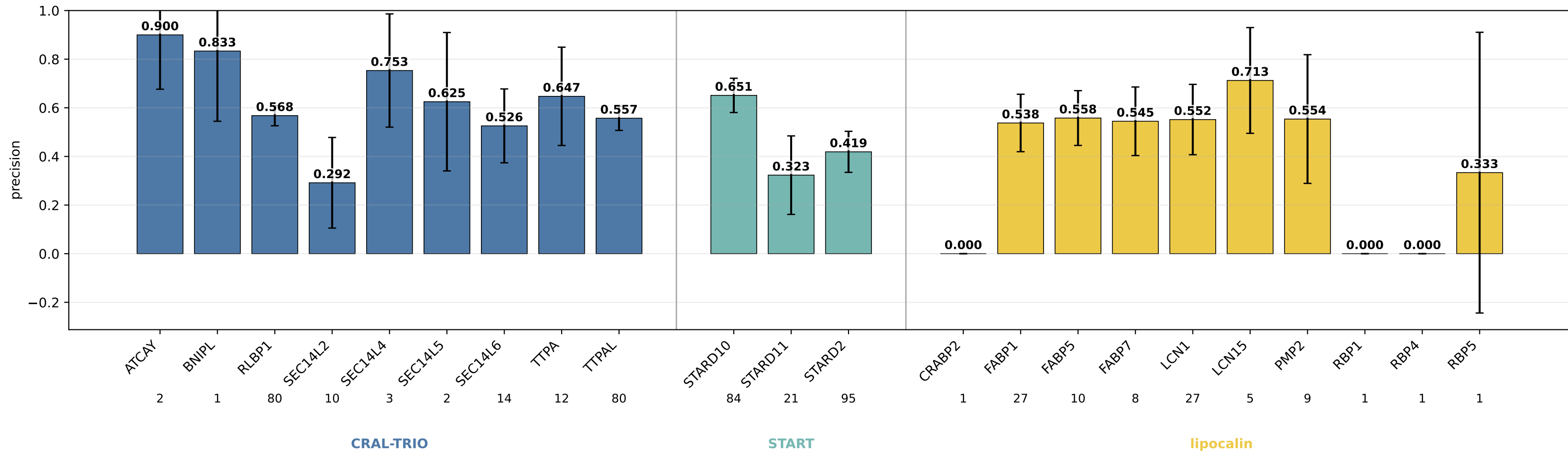
bbp_nps3mlp_dpt01_gm_pu01 precision by subgroup bbp_nps3mlp_dpt01_gm_pu01 | class weights | lr=0.0001 | weight_decay=1e-05 | final_m=4 | final_dropout=0.1 | hiddim=64 | heads=8 | batch=16 | ep=150 | seeds=0,1,2,3,4
