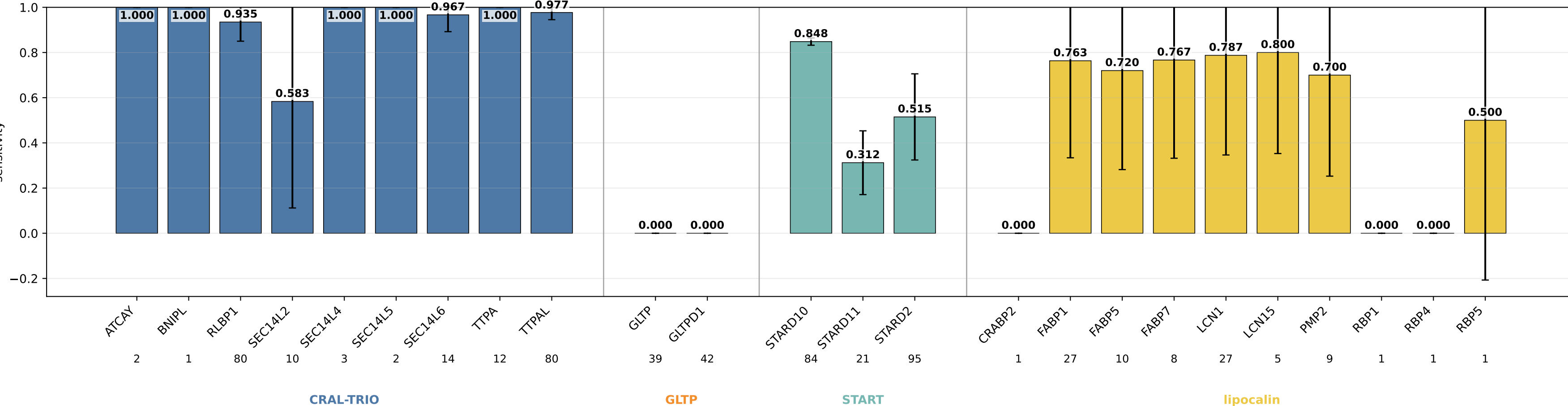
bbp_nps3mlp_dpt01_gm_pu01 sensitivity by subgroup bbp_nps3mlp_dpt01_gm_pu01 | class weights | lr=0.0001 | weight_decay=1e-05 | final_m=4 | final_dropout=0.1 | hiddim=64 | heads=8 | batch=16 | ep=150 | seeds=0,1,2,3,4
