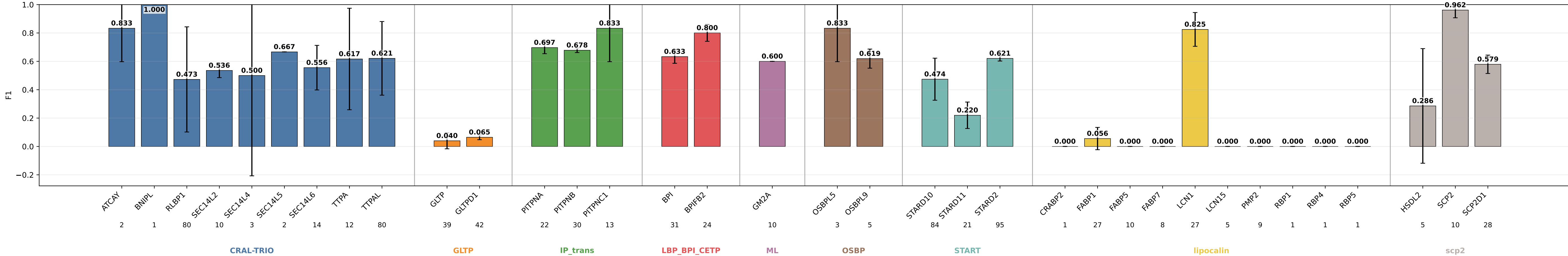
bbp_nps3mlp_dpt01_wd0001_gm_plm64_hid64 F1 by subgroup bbp_nps3mlp_dpt01_wd0001_gm_plm64_hid64 | class weights | lr=0.0001 | weight_decay=0.001 | final_m=4 | final_dropout=0.1 | hiddim=64 | heads=8 | batch=16 | ep=150 | seeds=0,1
