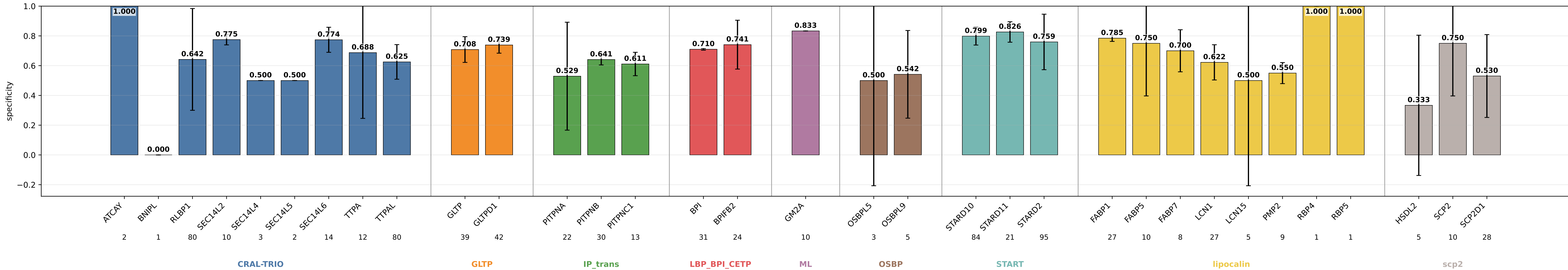
bbp_nps3mlp_dpt01_wd0001_gm_plm64_hid64_GRL specificity by subgroup bbp_nps3mlp_dpt01_wd0001_gm_plm64_hid64_GRL | class weights | lr=0.0001 | weight_decay=0.001 | final_m=4 | final_dropout=0.1 | hiddim=64 | heads=8 | batch=16 | ep=150 | seeds=0,1
