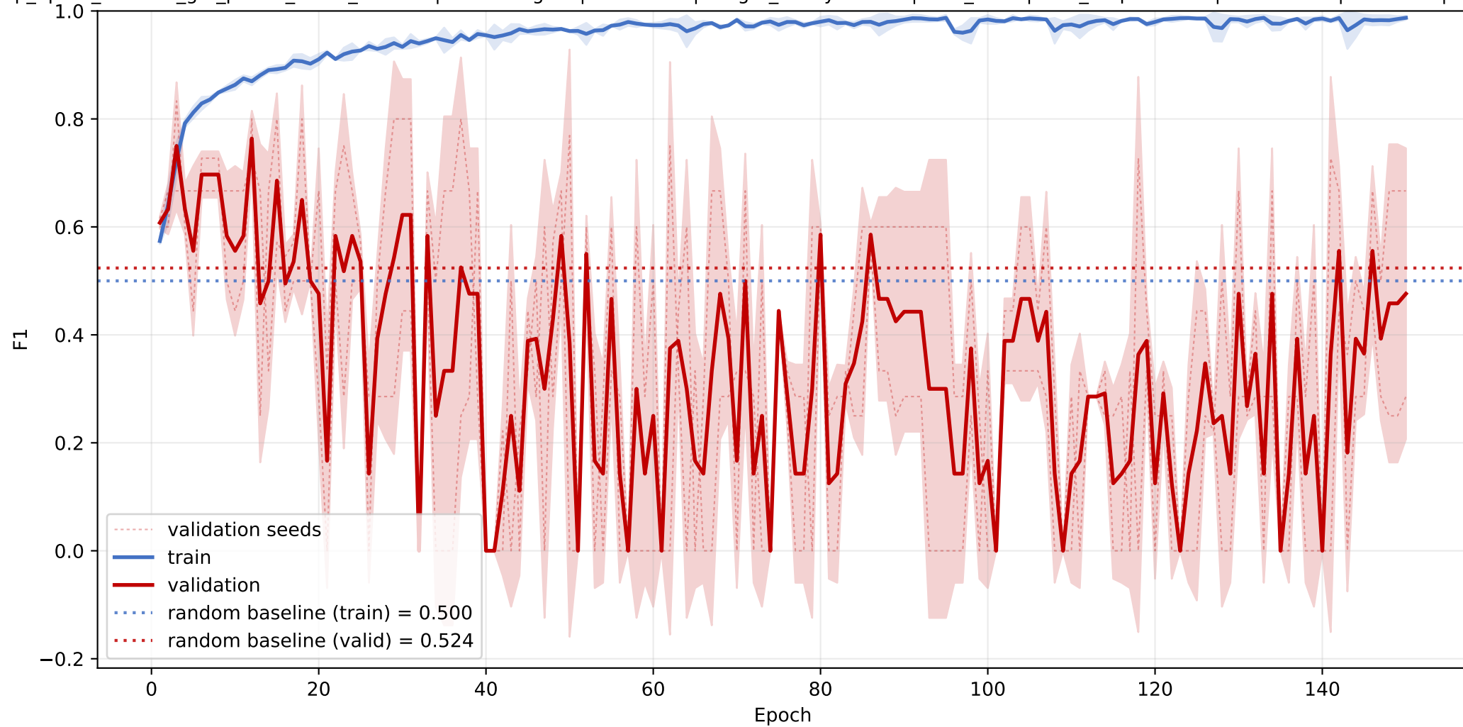
ML: mean F1 learning curve across seeds
