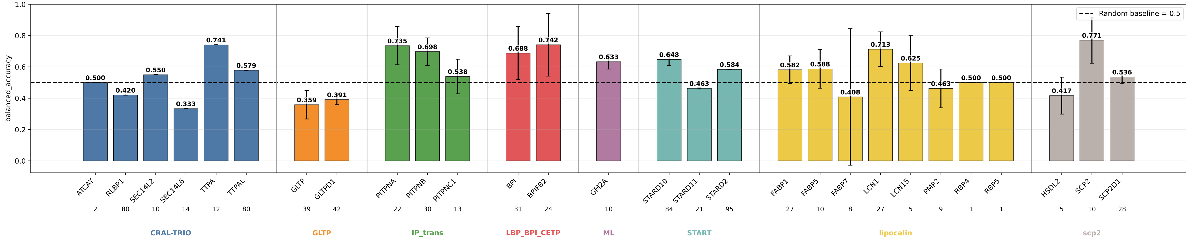
bbp_nps3mlp_dpt01_wd0001_gm_plm64_hid64_bilinear balanced_accuracy by subgroup bbp_nps3mlp_dpt01_wd0001_gm_plm64_hid64_bilinear | class weights | lr=0.0001 | weight_decay=0.001 | final_m=4 | final_dropout=0.1 | hiddim=64 | heads=8 | batch=16 | ep=150 | seeds=0,1
