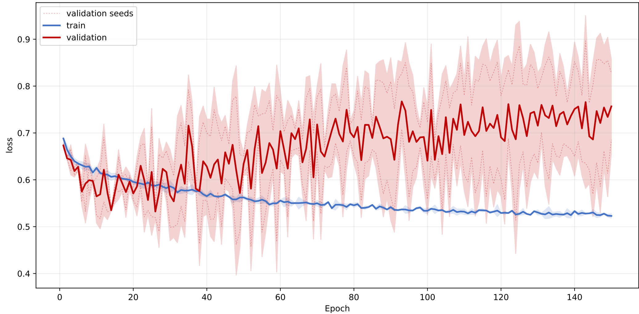
ML: mean loss learning curve across seeds
