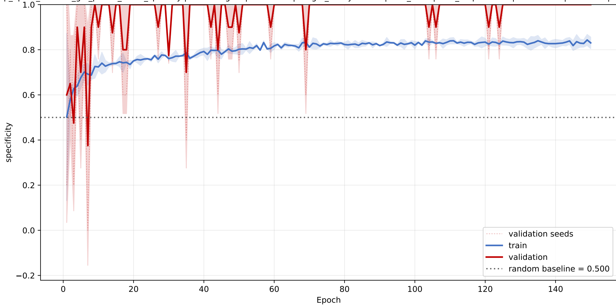
ML: mean specificity learning curve across seeds
