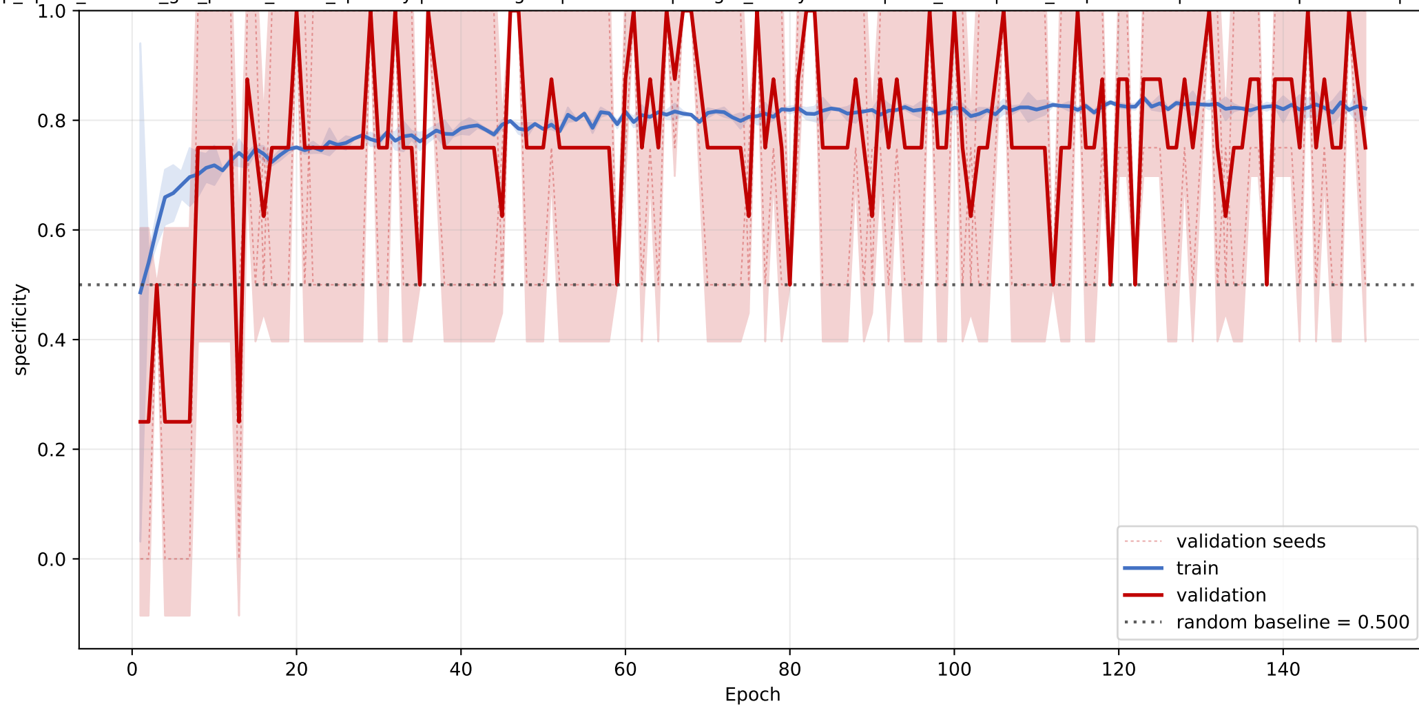
OSBP: mean specificity learning curve across seeds
