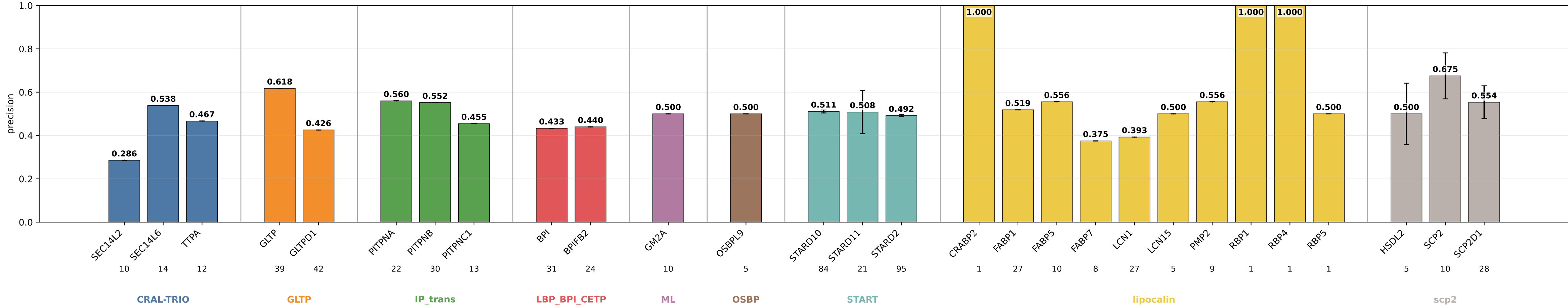
bbp_nps3mlp_dpt01_wd0001_gm_plm64_hid64_protonly precision by subgroup bbp_nps3mlp_dpt01_wd0001_gm_plm64_hid64_protonly | class weights | lr=0.0001 | weight_decay=0.001 | final_m=4 | final_dropout=0.1 | hiddim=64 | heads=8 | batch=16 | ep=150 | seeds=0,1
