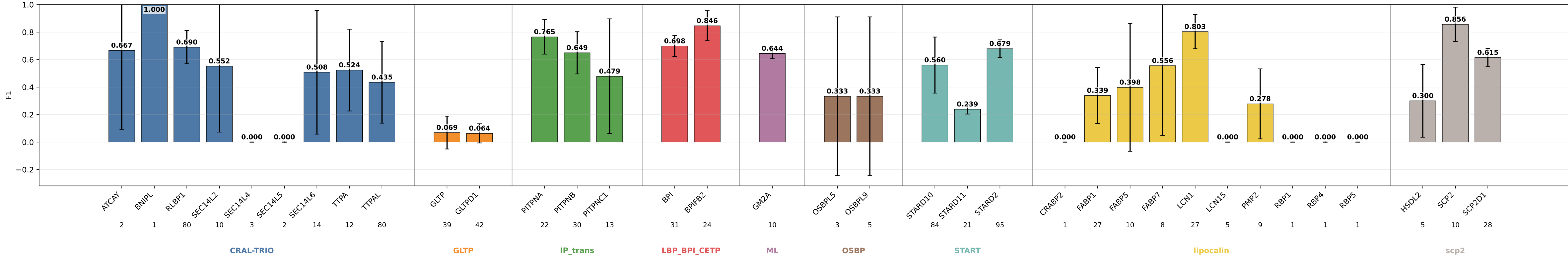
bbp_nps3mlp_esmv2_dpt01_wd0001_ap_plm64_hid64 F1 by subgroup bbp_nps3mlp_esmv2_dpt01_wd0001_ap_plm64_hid64 | class weights | lr=0.0001 | weight_decay=0.001 | final_m=4 | final_dropout=0.1 | hiddim=64 | heads=8 | batch=16 | ep=150 | seeds=0,1,2
