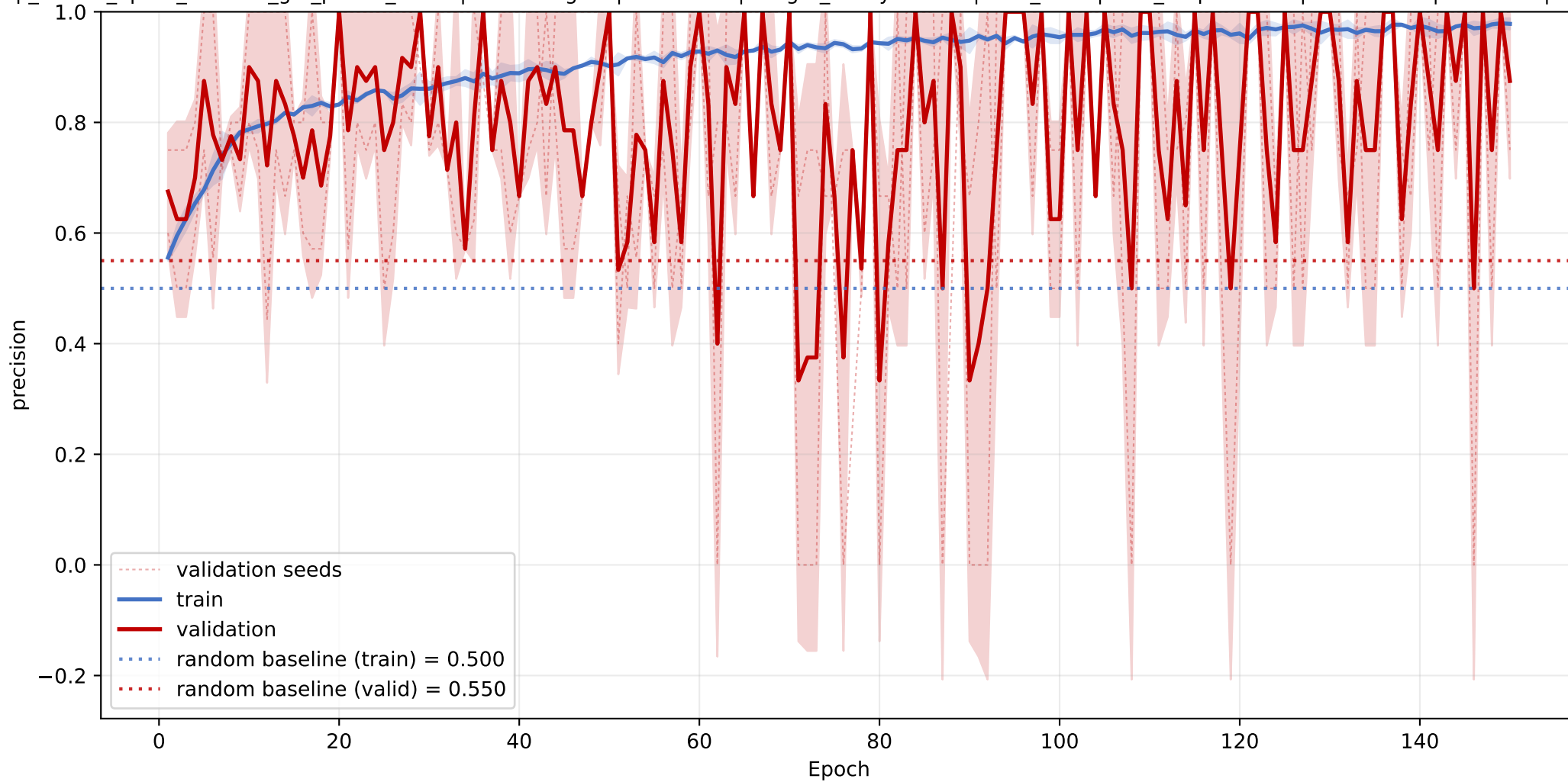
ML: mean precision learning curve across seeds
