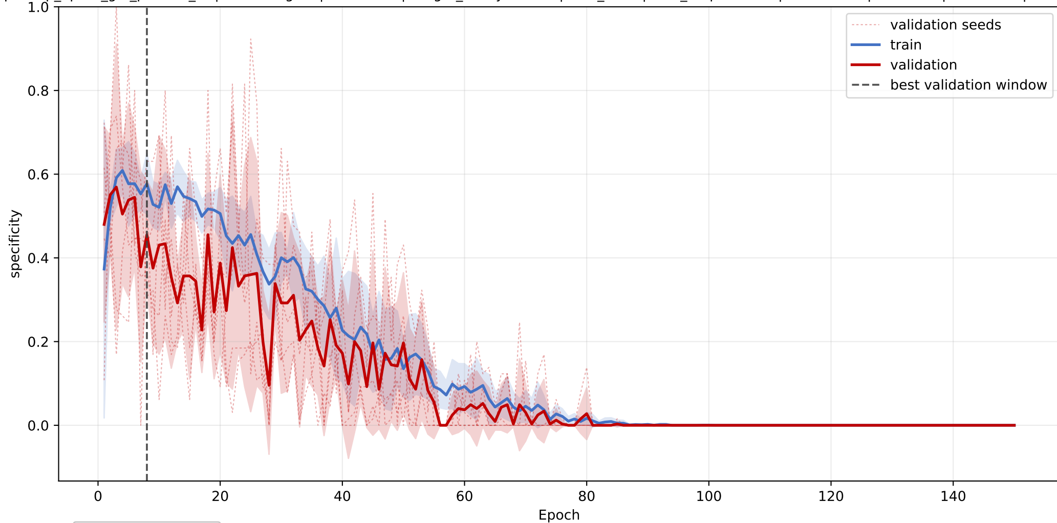
CRAL-TRIO-IP_trans: mean specificity learning curve across seeds
