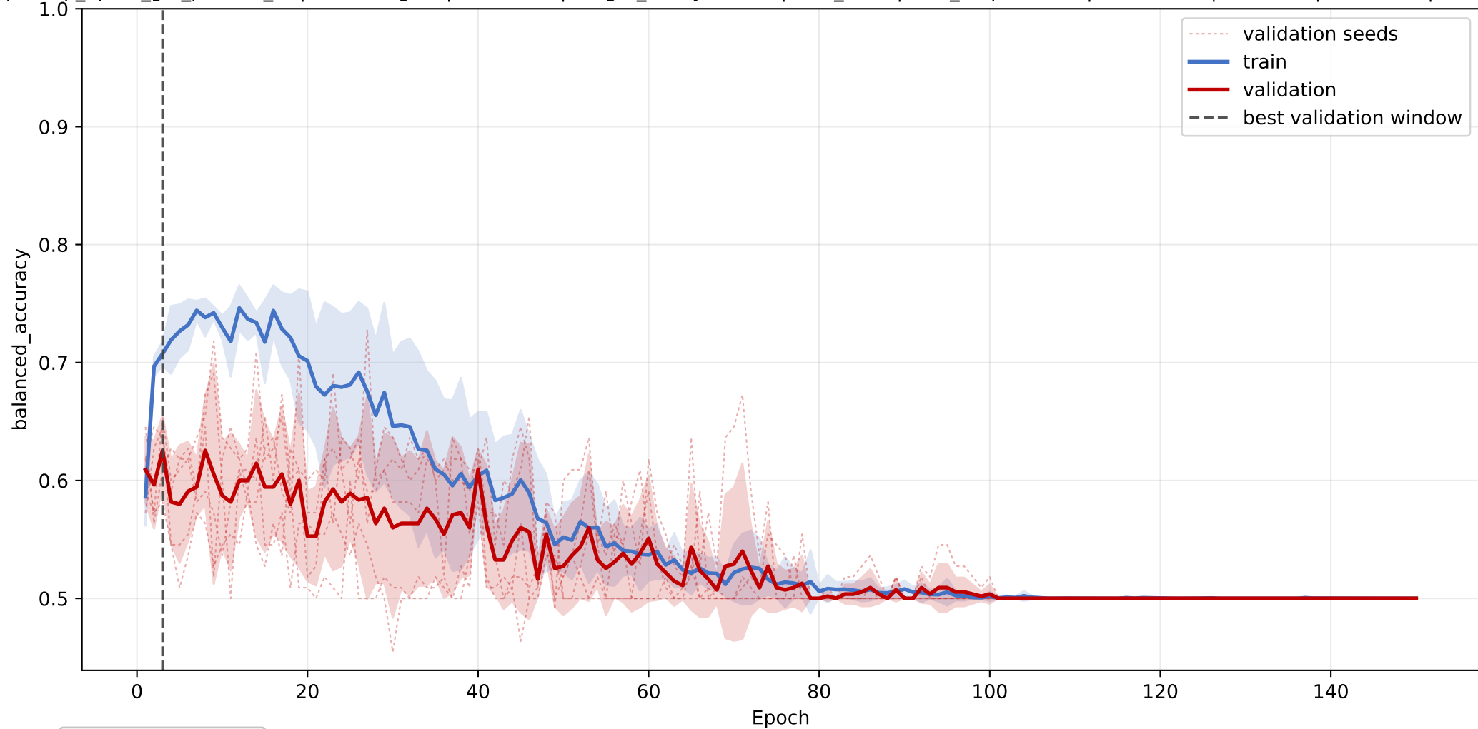
GLTP-LBP_BPI_CETP: mean balanced_accuracy learning curve across seeds
