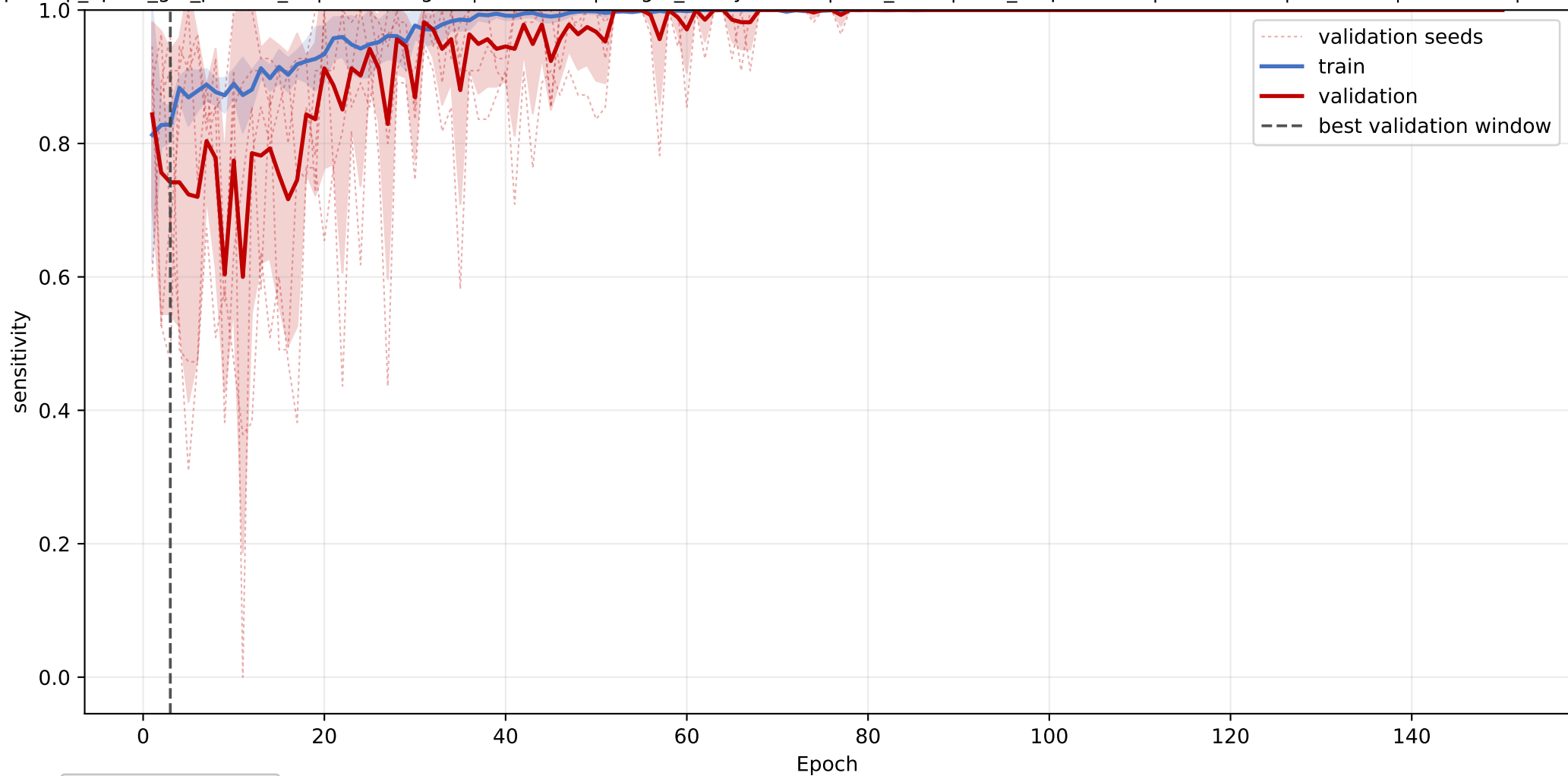
GLTP-LBP_BPI_CETP: mean sensitivity learning curve across seeds
