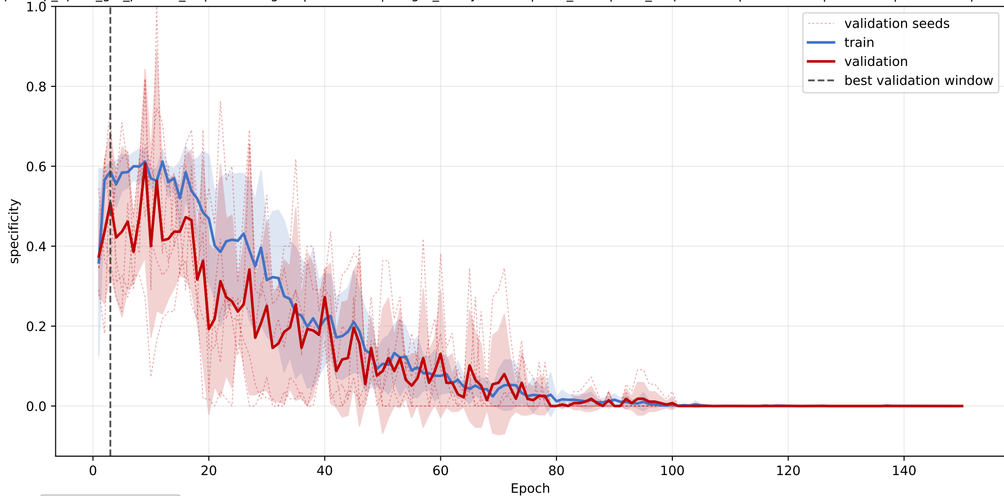
GLTP-LBP_BPI_CETP: mean specificity learning curve across seeds
