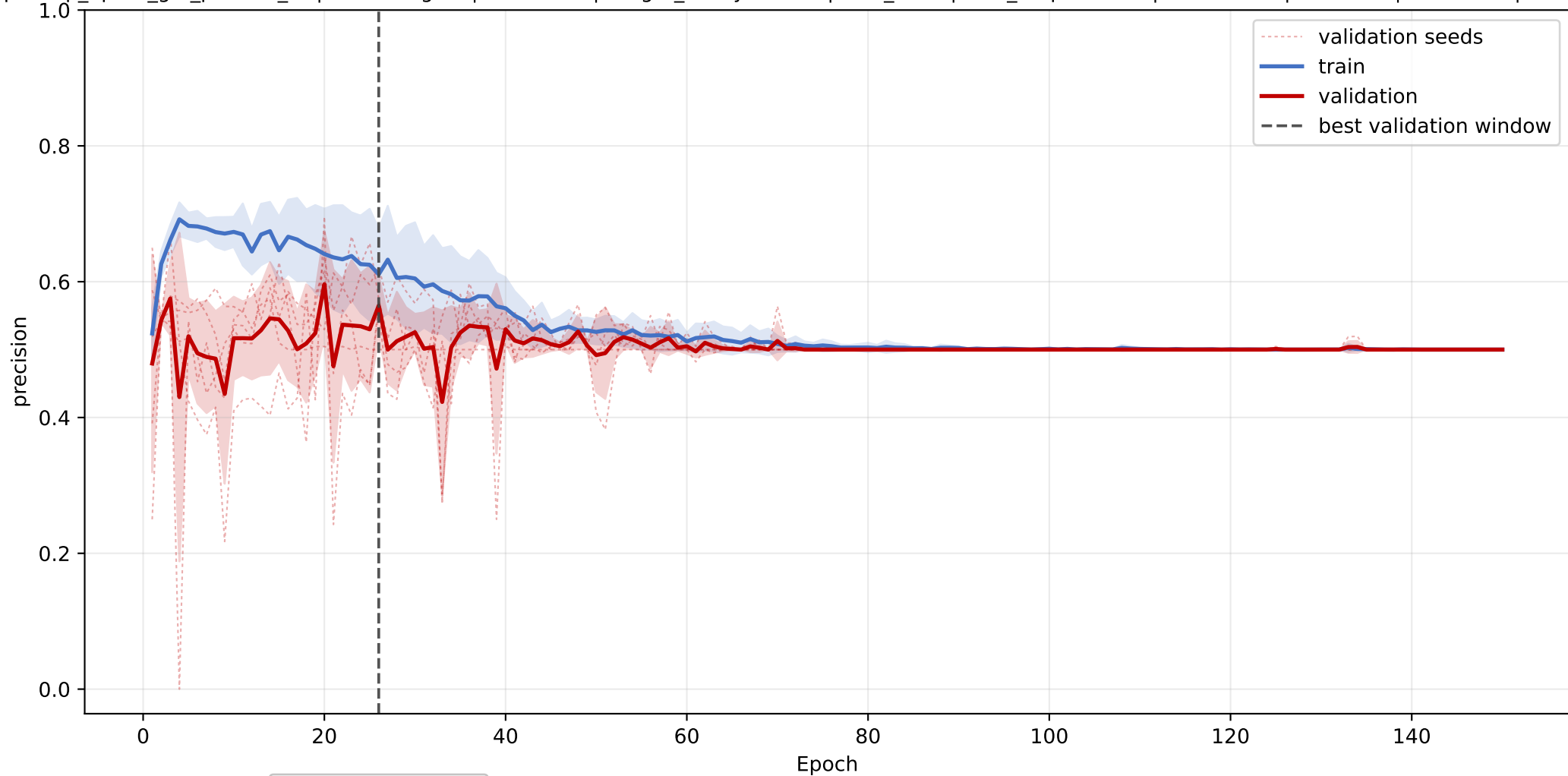
IP_trans-LBP_BPI_CETP: mean precision learning curve across seeds
