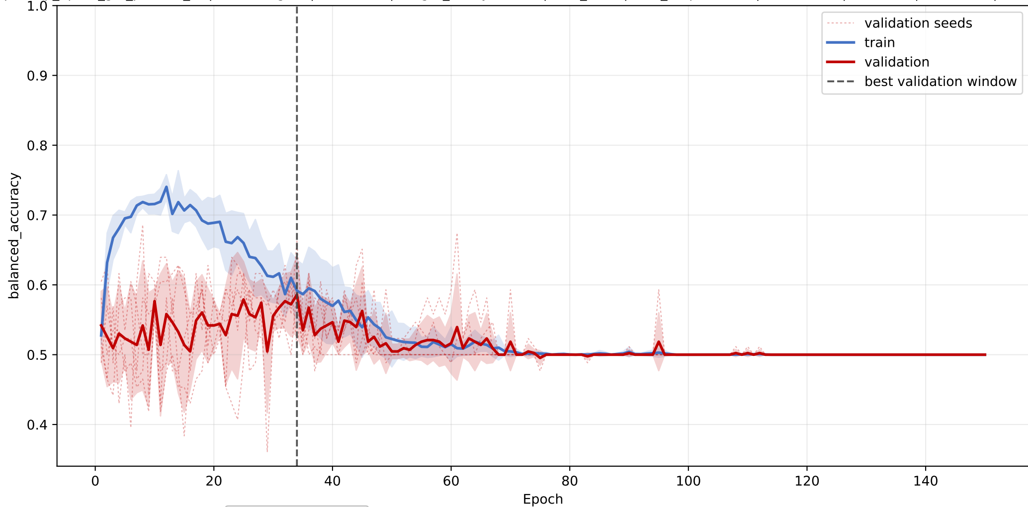
ML-scp2: mean balanced_accuracy learning curve across seeds
