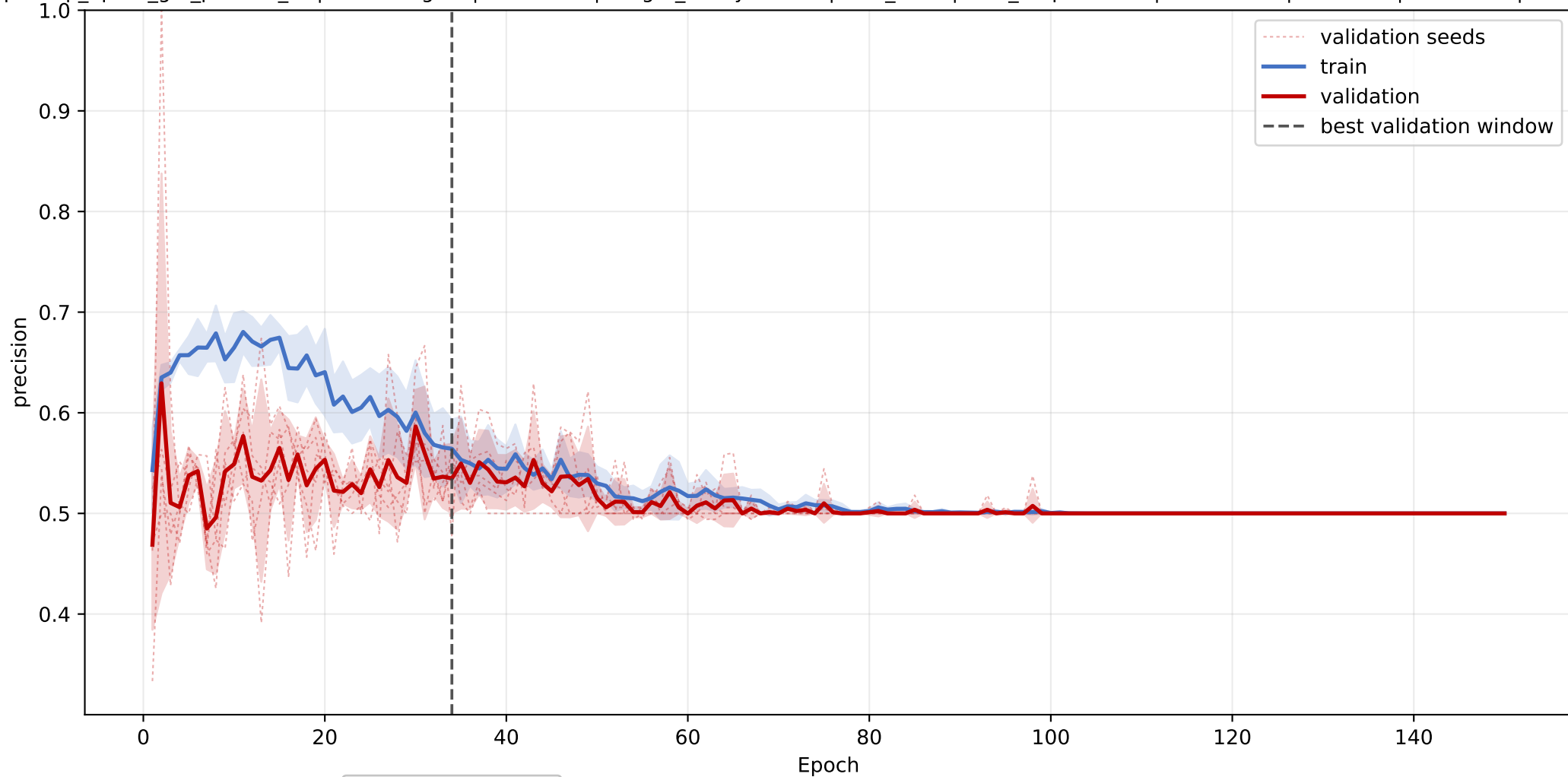
OSBP-scp2: mean precision learning curve across seeds
