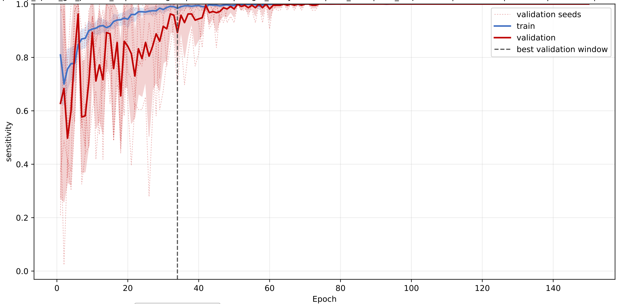
OSBP-scp2: mean sensitivity learning curve across seeds
