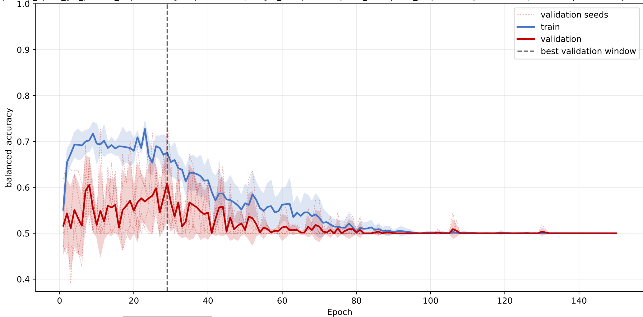
START-LBP_BPI_CETP: mean balanced_accuracy learning curve across seeds
