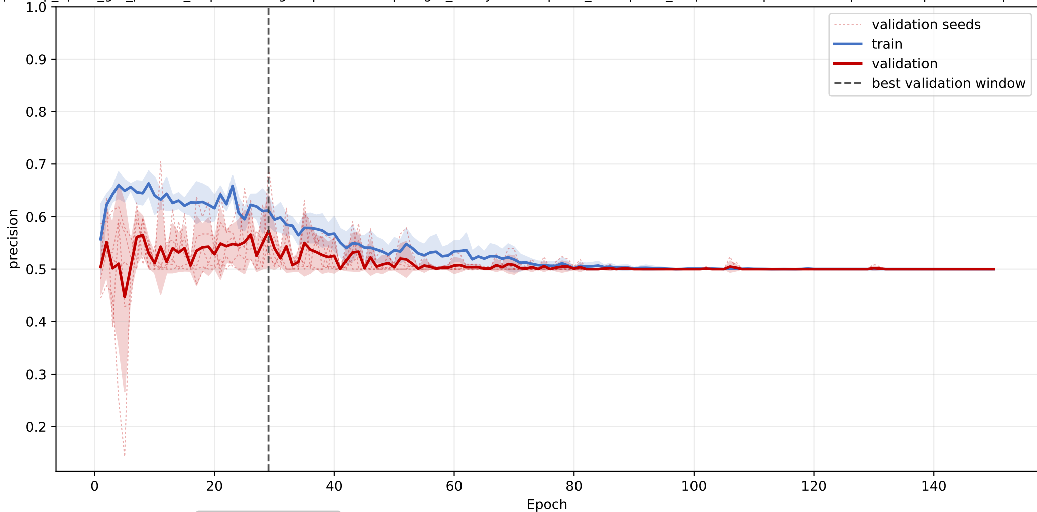
START-LBP_BPI_CETP: mean precision learning curve across seeds
