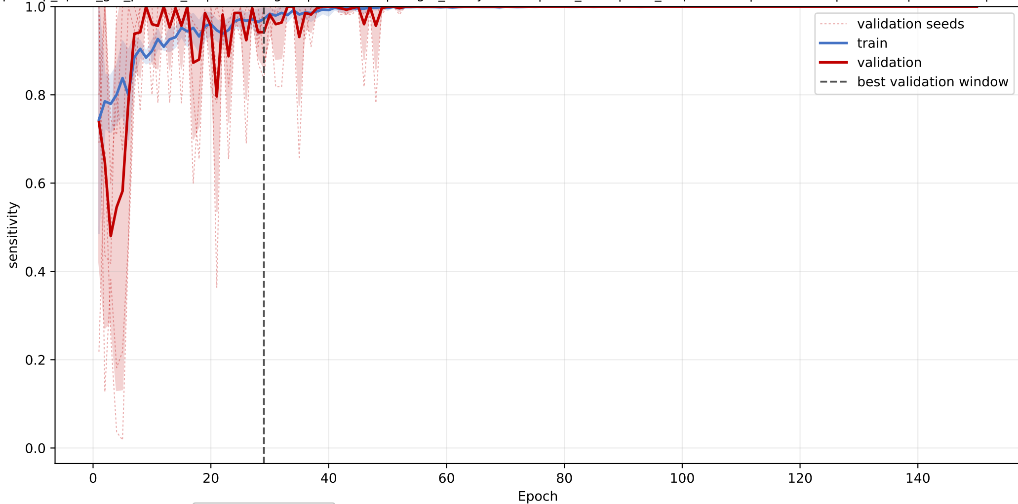
START-LBP_BPI_CETP: mean sensitivity learning curve across seeds
