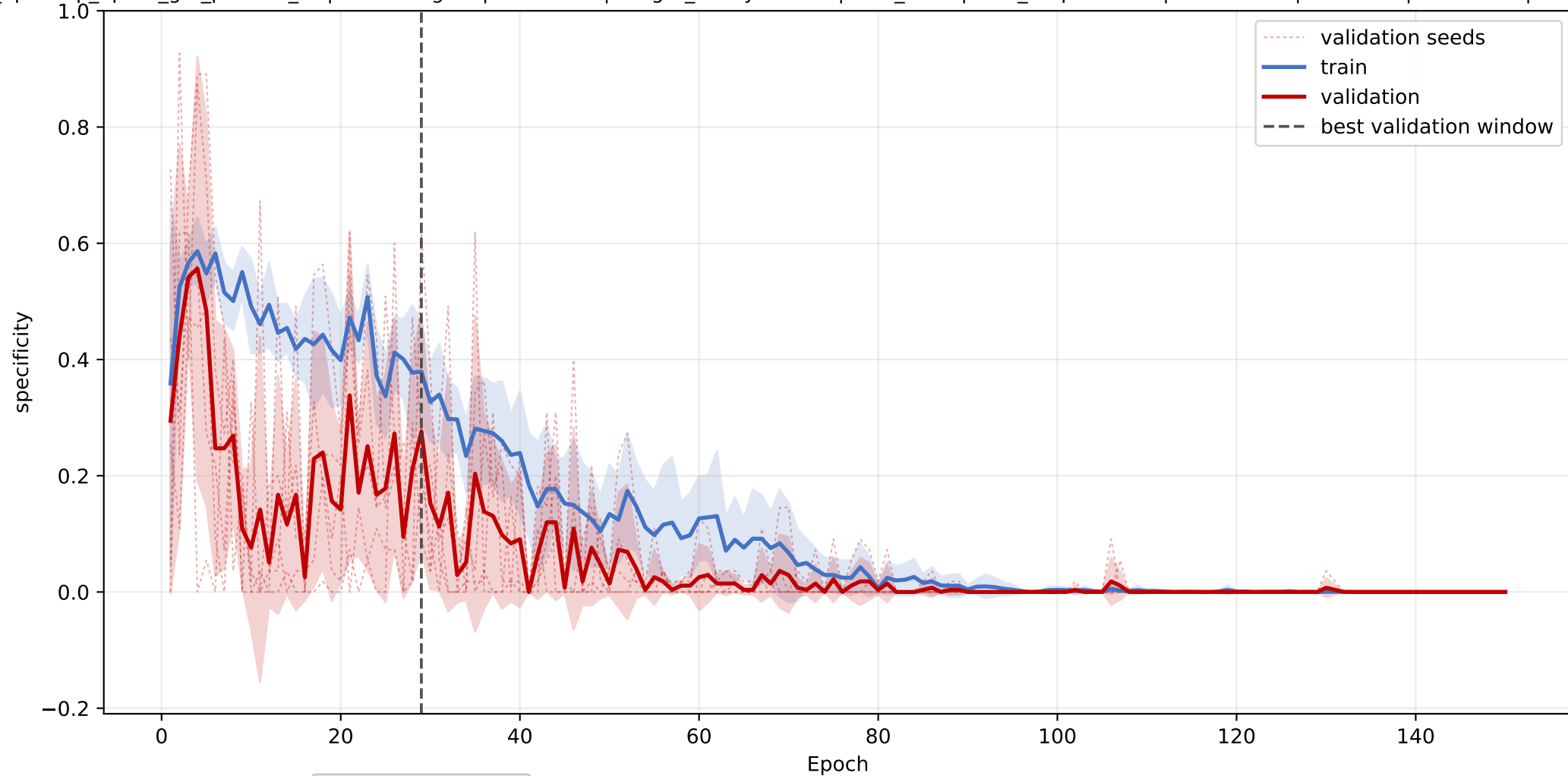
START-LBP_BPI_CETP: mean specificity learning curve across seeds
