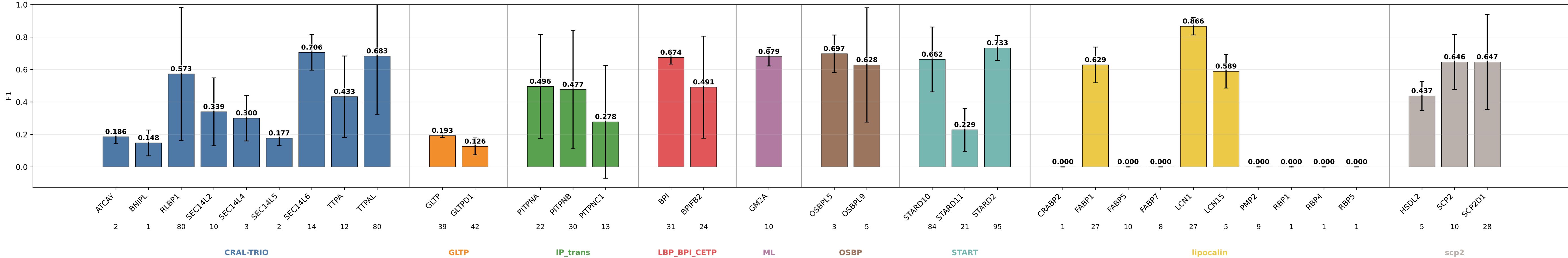
bf_nps3mlp_dpt01_gm_pu0025_cs F1 by subgroup bf_nps3mlp_dpt01_gm_pu0025_cs | class weights | lr=0.0001 | weight_decay=1e-05 | final_m=4 | final_dropout=0.1 | hiddim=64 | heads=8 | batch=16 | ep=150 | seeds=0,1,2,3,4
