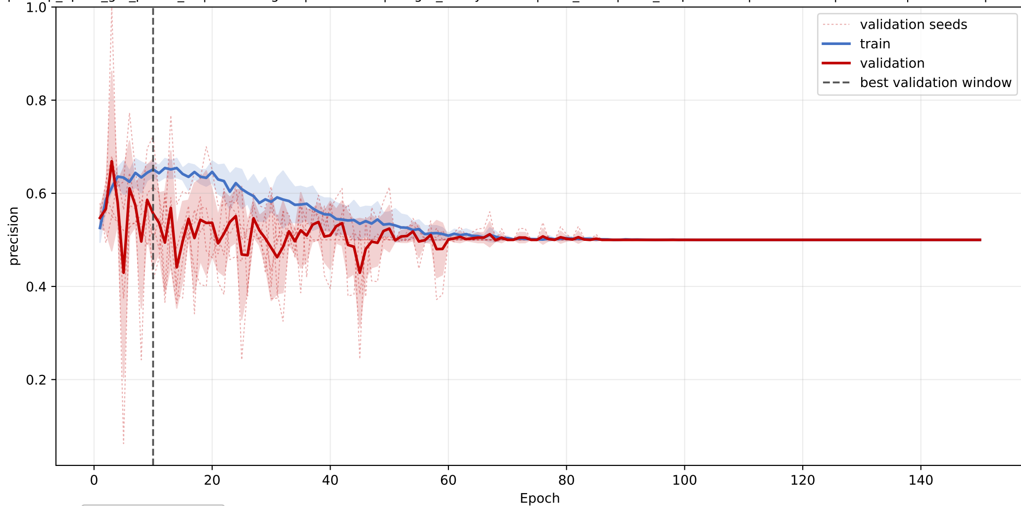
CRAL-TRIO-IP_trans: mean precision learning curve across seeds
