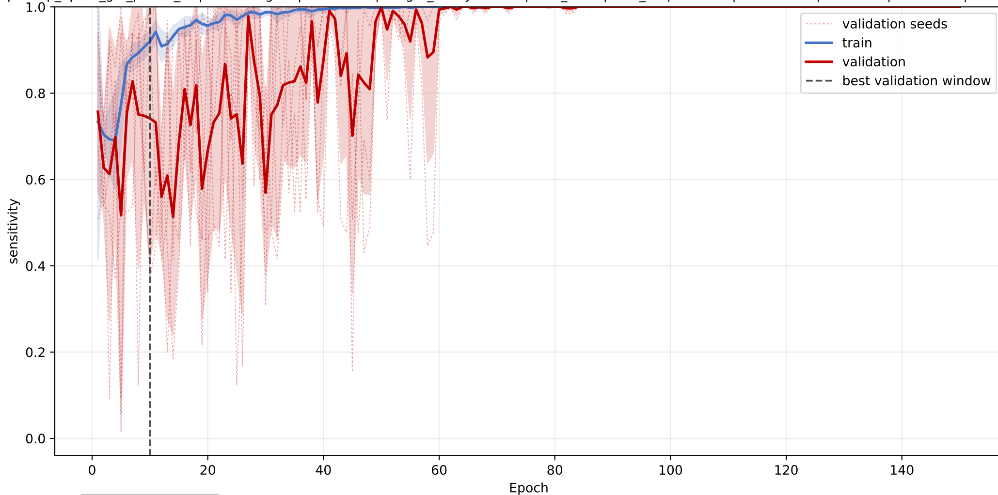
CRAL-TRIO-IP_trans: mean sensitivity learning curve across seeds
