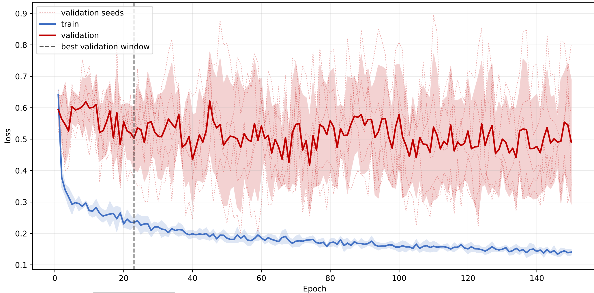
GLTP-LBP_BPI_CETP: mean loss learning curve across seeds
