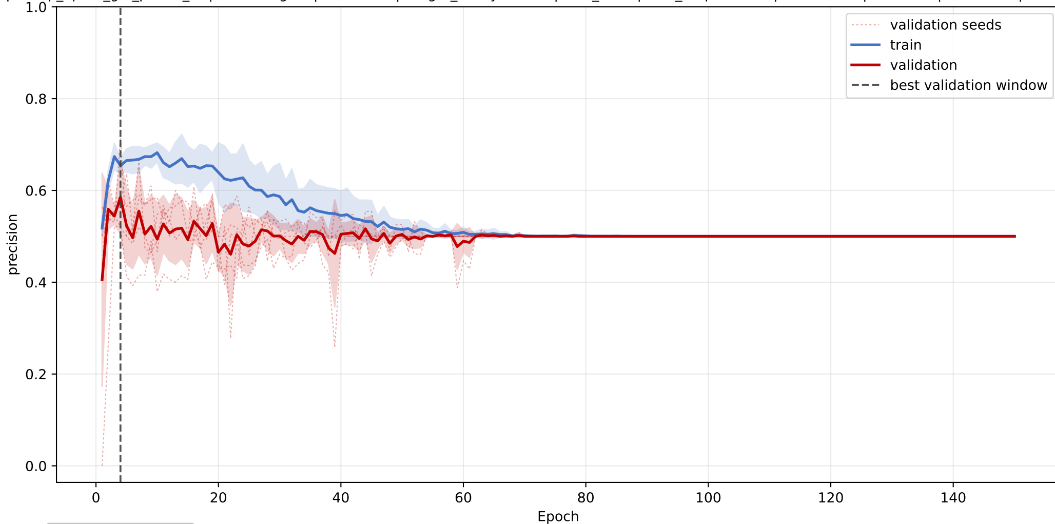
IP_trans-LBP_BPI_CETP: mean precision learning curve across seeds
