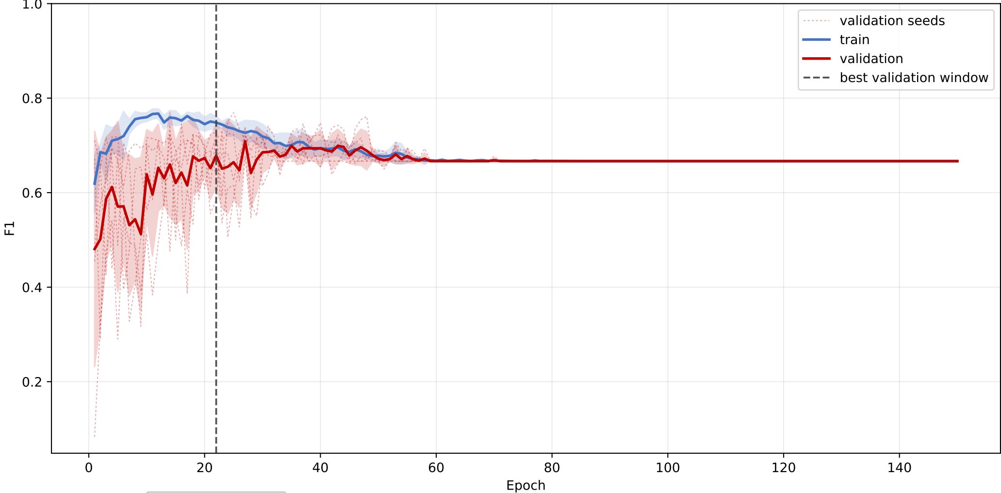
ML-scp2: mean F1 learning curve across seeds
