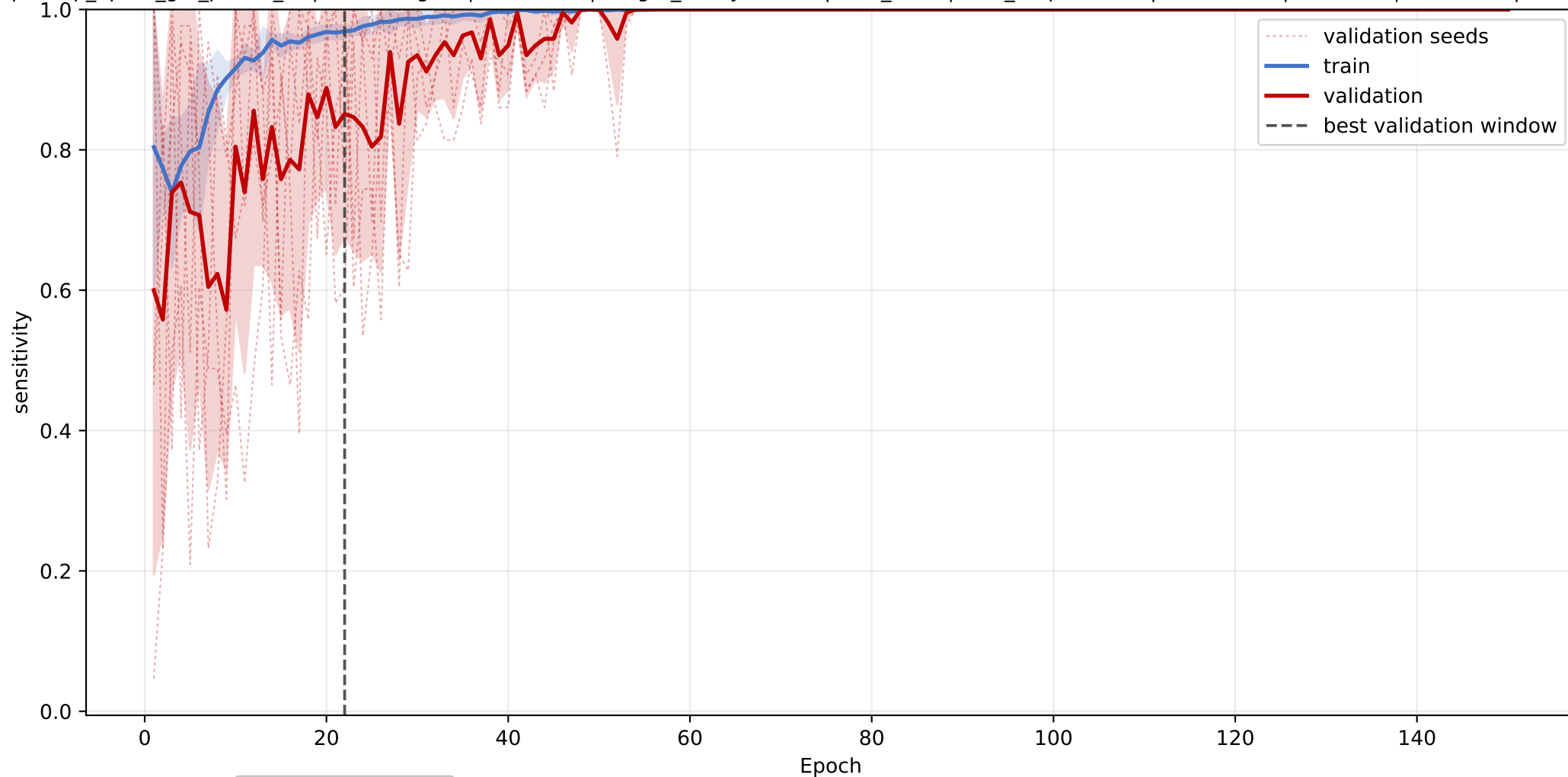
ML-scp2: mean sensitivity learning curve across seeds
